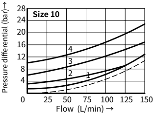
\Delta P -Q curves – sub plate mounting
