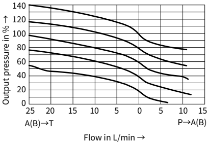
Pressure-flow relationship
